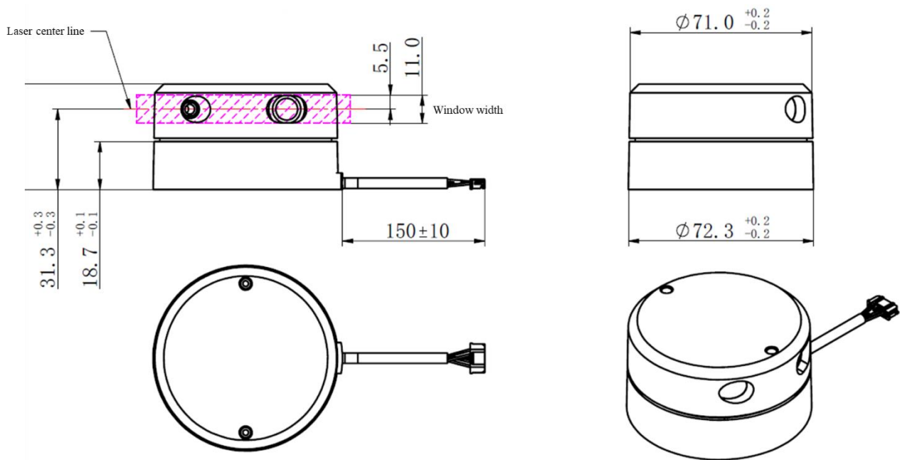
FIG 1 YDLIDAR G4 INSTALLATION&MECHANICAL SIZE (UNIT:MM)
