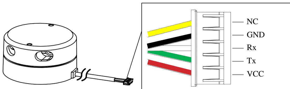
FIG 2 YDLIDAR G4 INTERFACES
