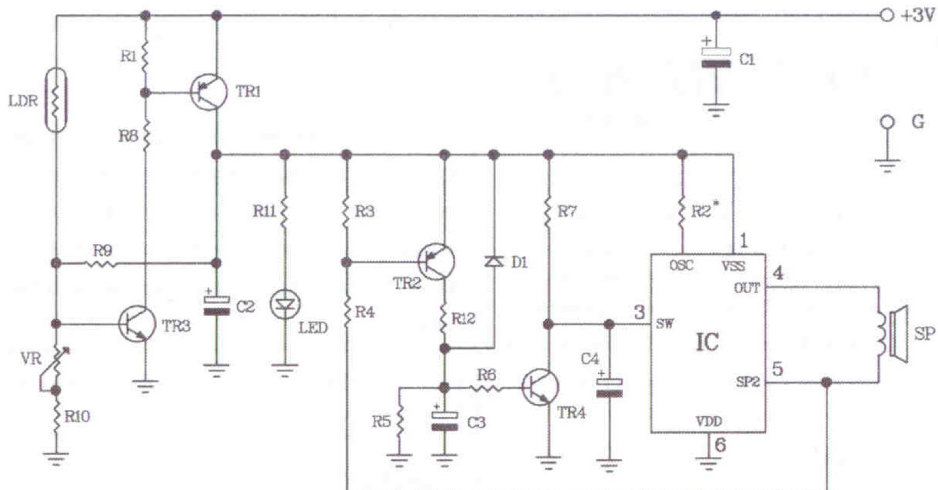
Figure 2. Light activate alarm (cock voice) circuit
