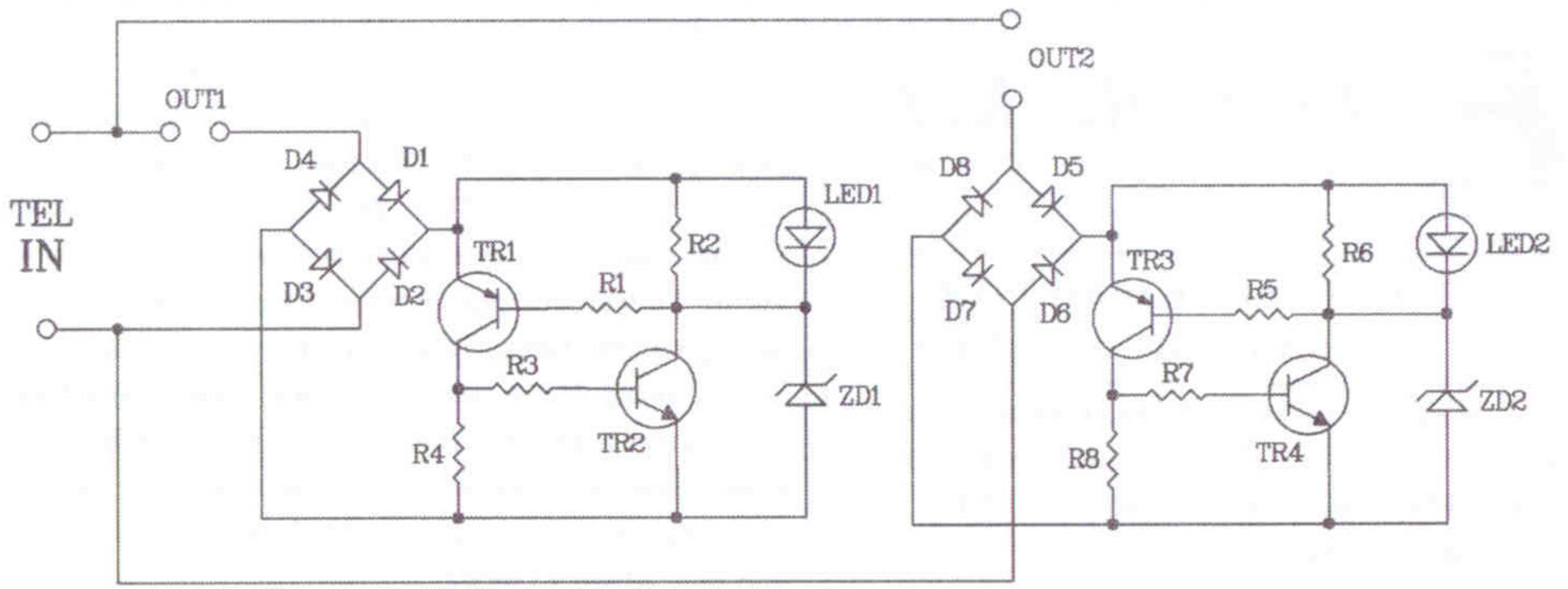
Figure 2. The telephone privacy protection circuit
