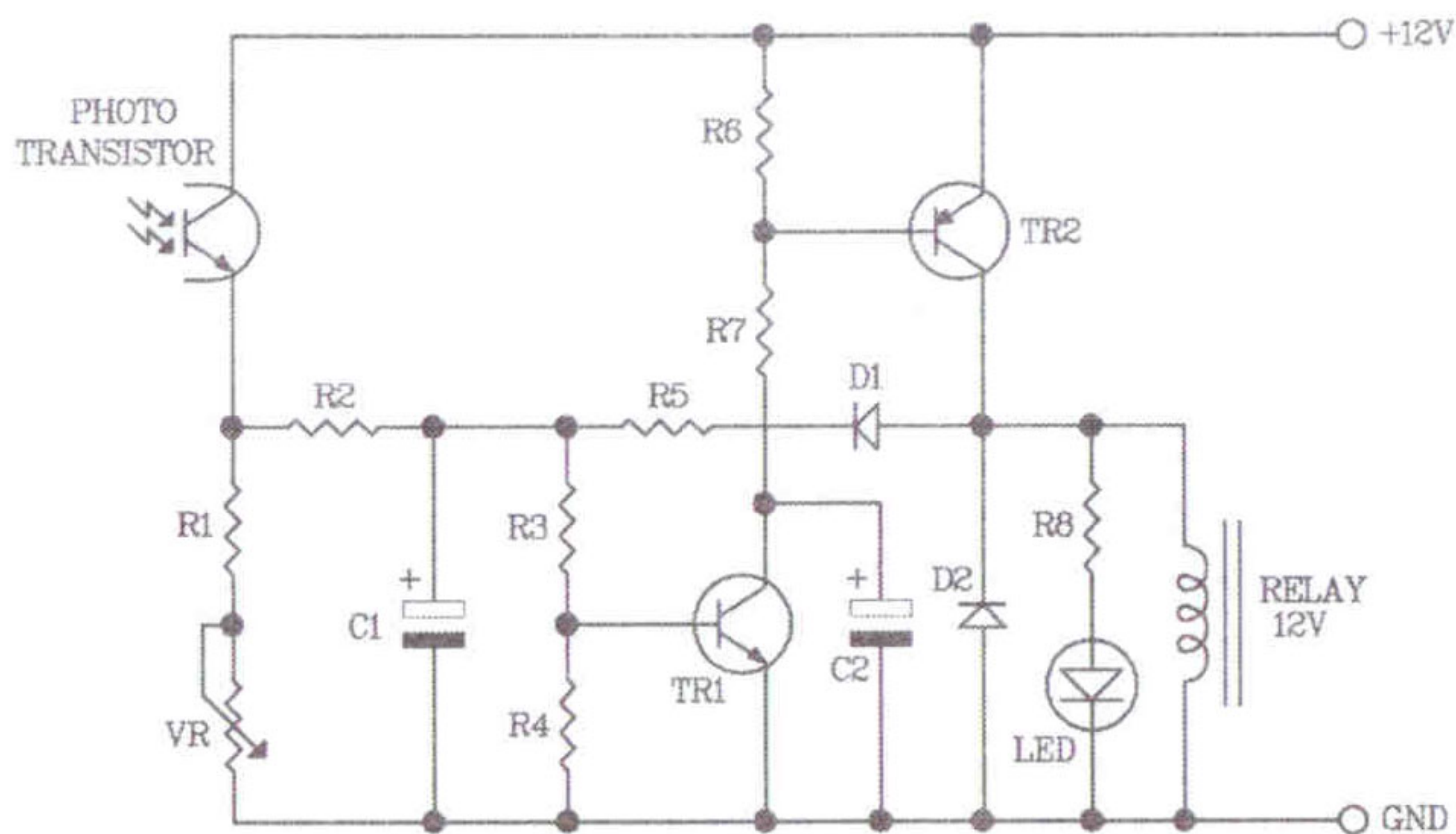
Figure 2. The light activate switch (light-on) circuit
