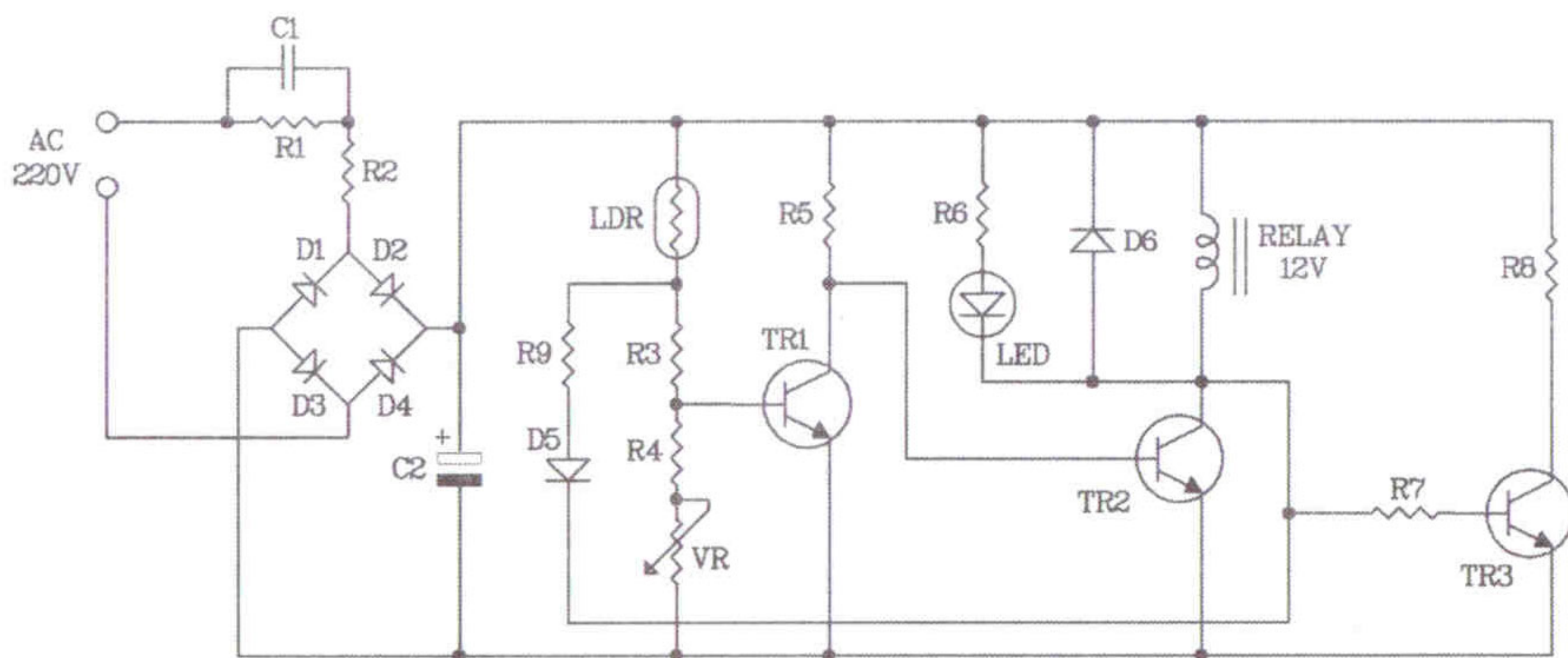
Figure 2. The night activate switch 220V. circuit
