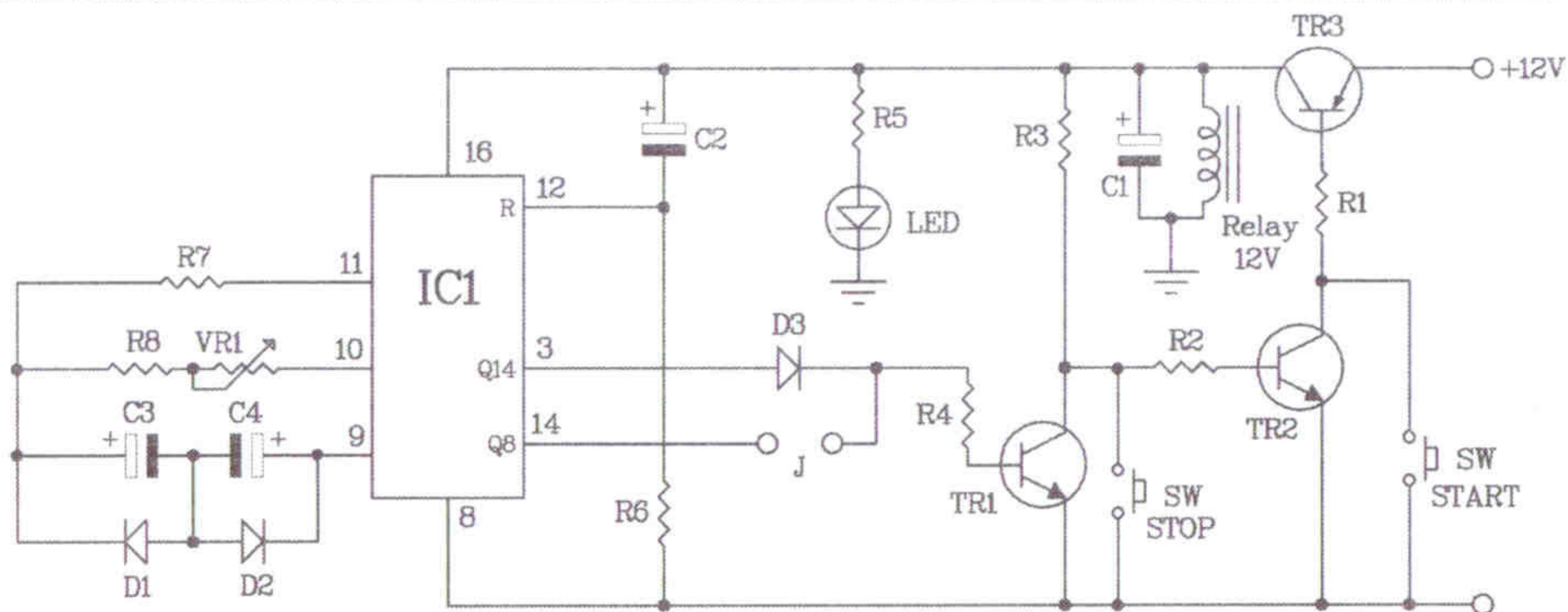
Figure 2. The timer switch 0-3 hr. circuit
