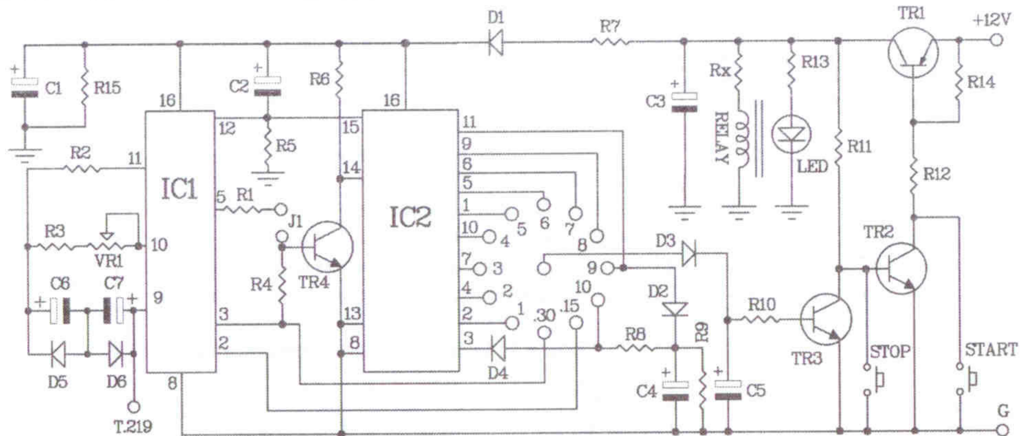
Figure 2. The timer switch 0-10hr. circuit
