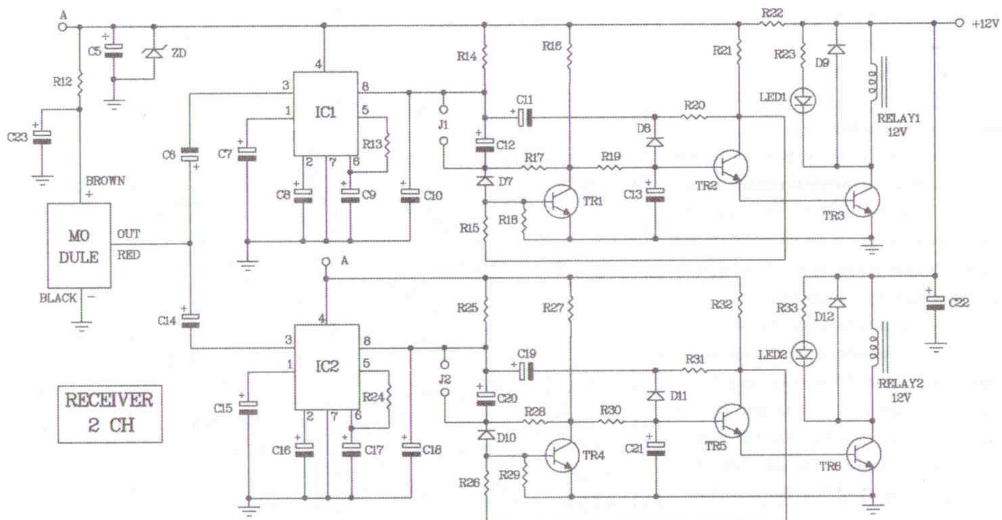
Figure 2. The infrared remote control 50' 2 ch. circuit
