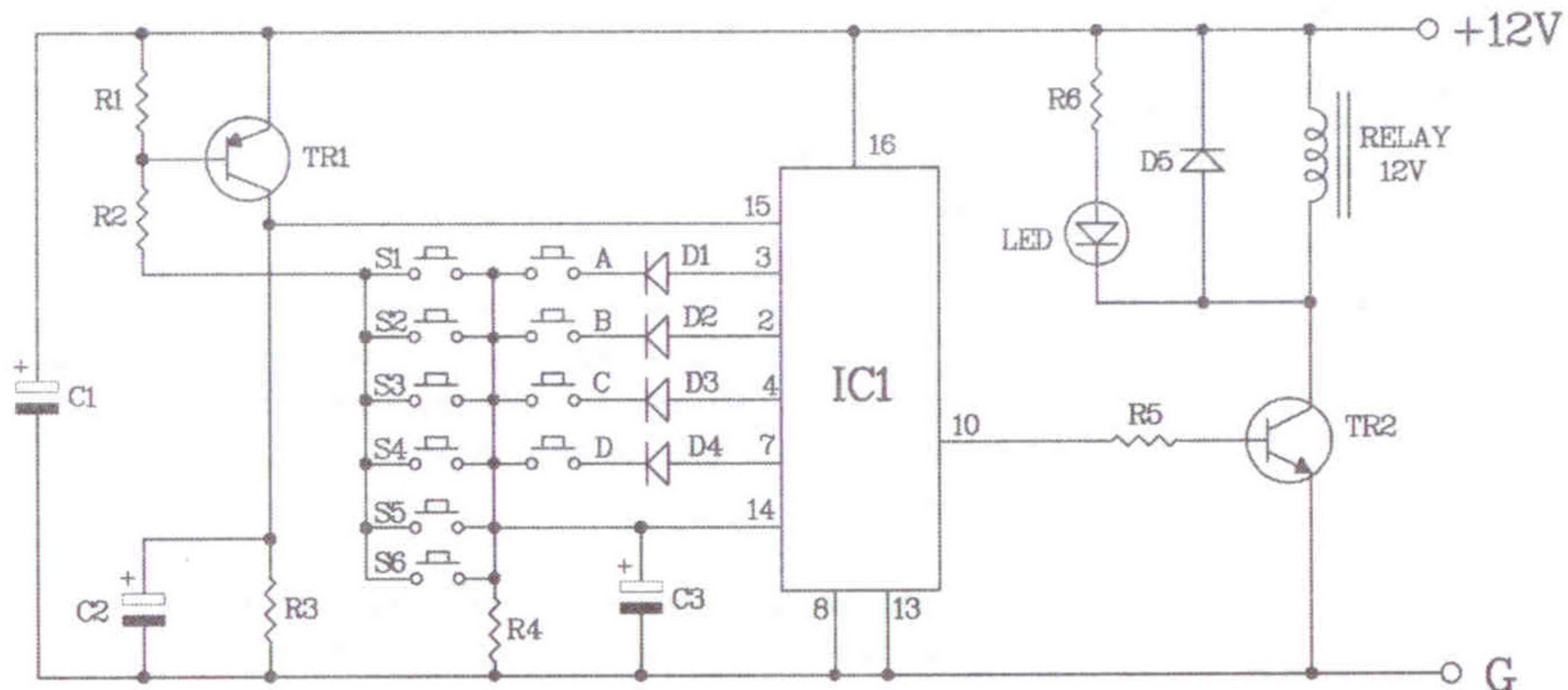
Figure 2. The electronic code switch circuit
