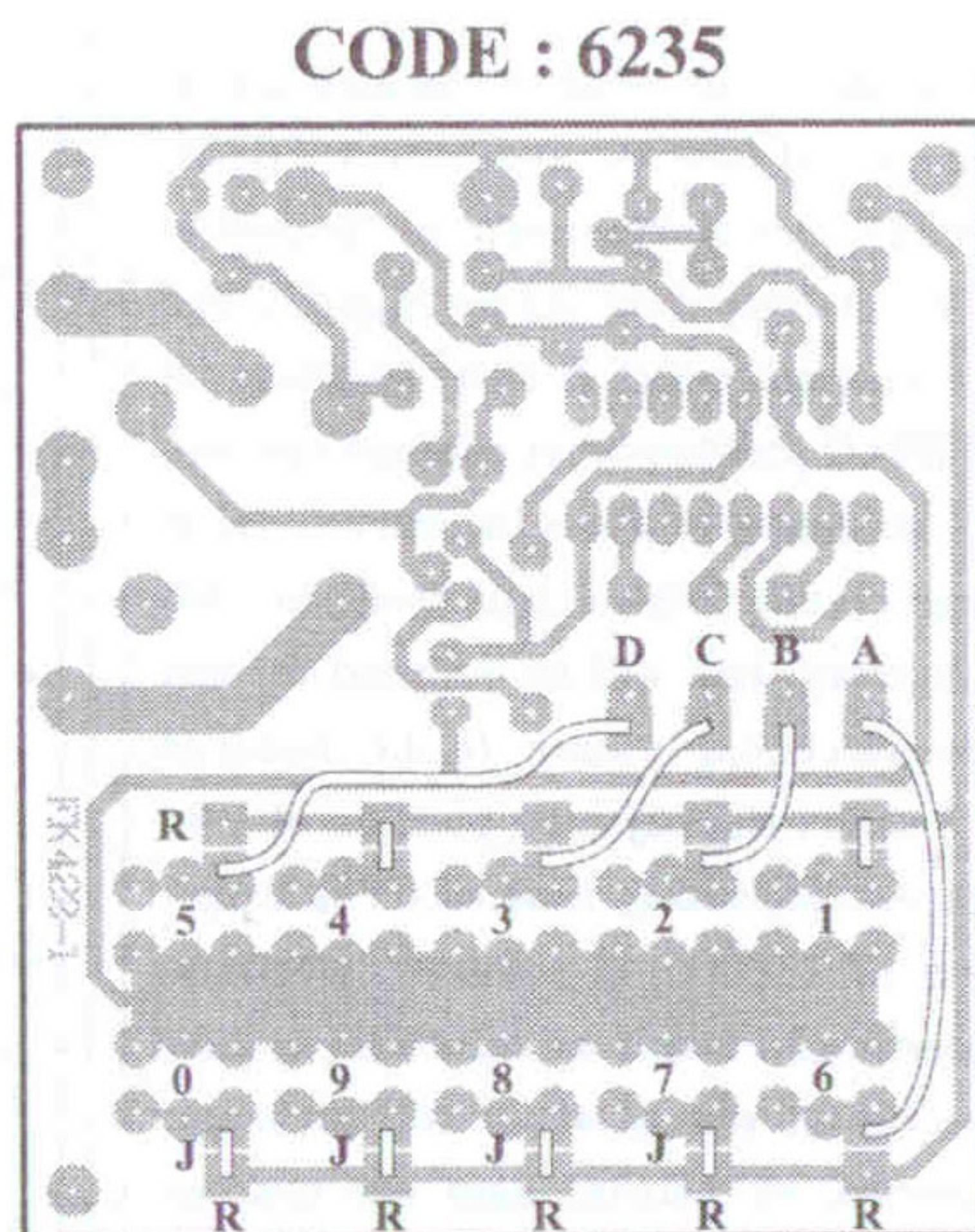
Figure 3. Connections
