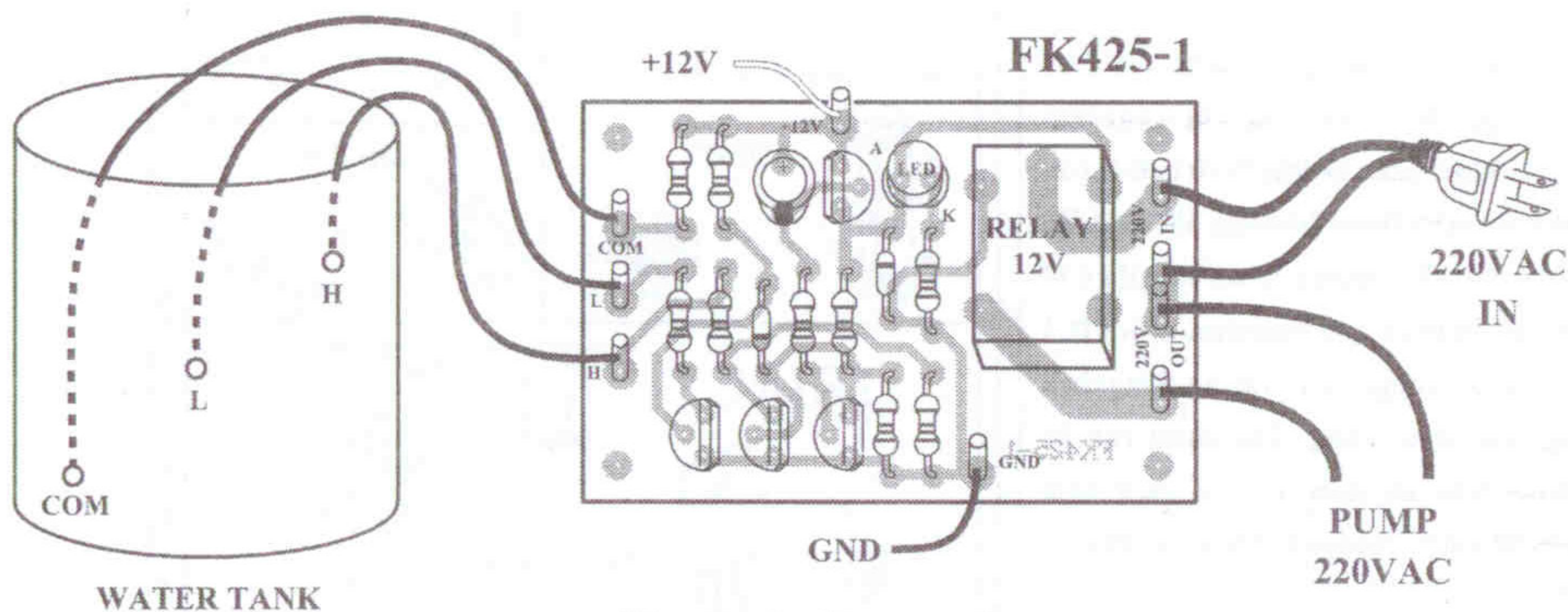
Figure 3. Connections
