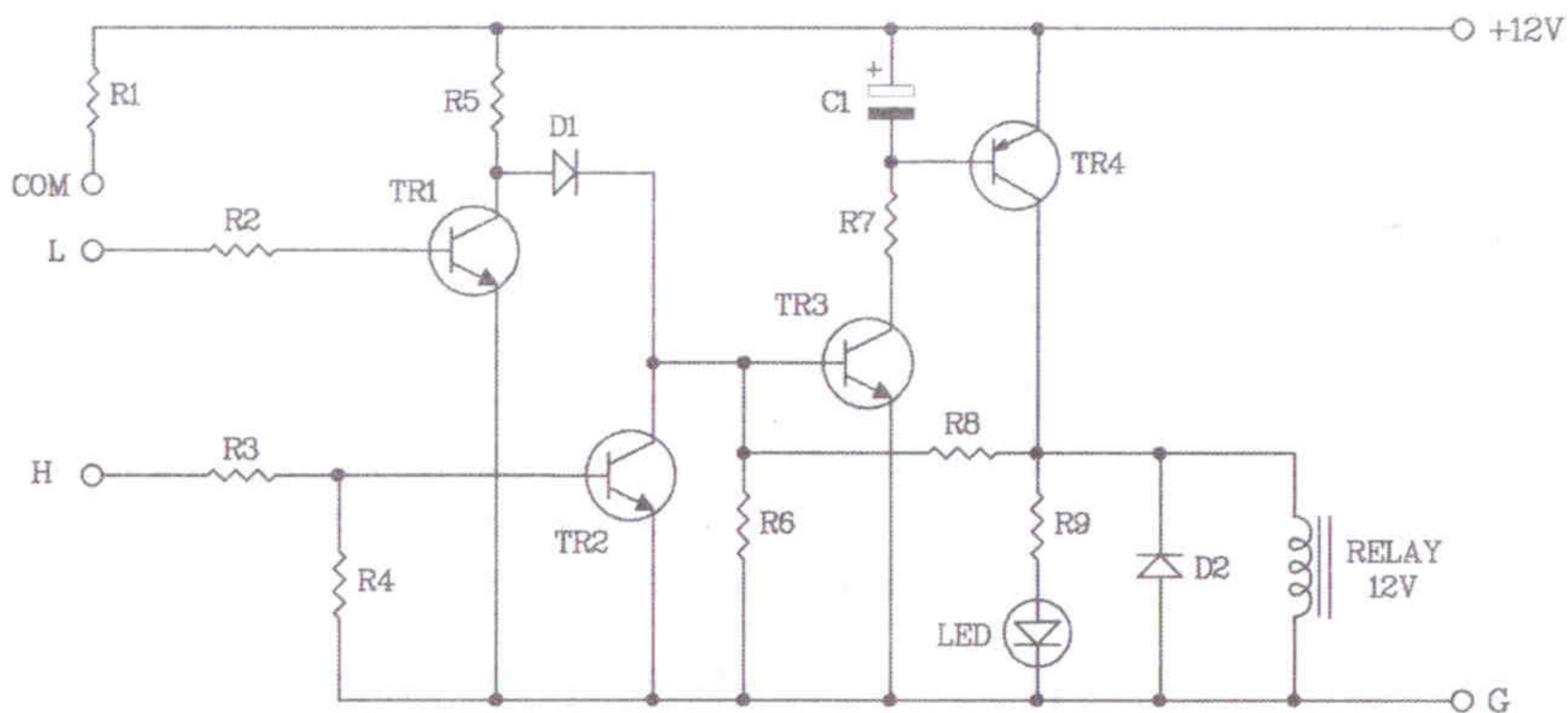
Figure 2. The water pump level control circuit
