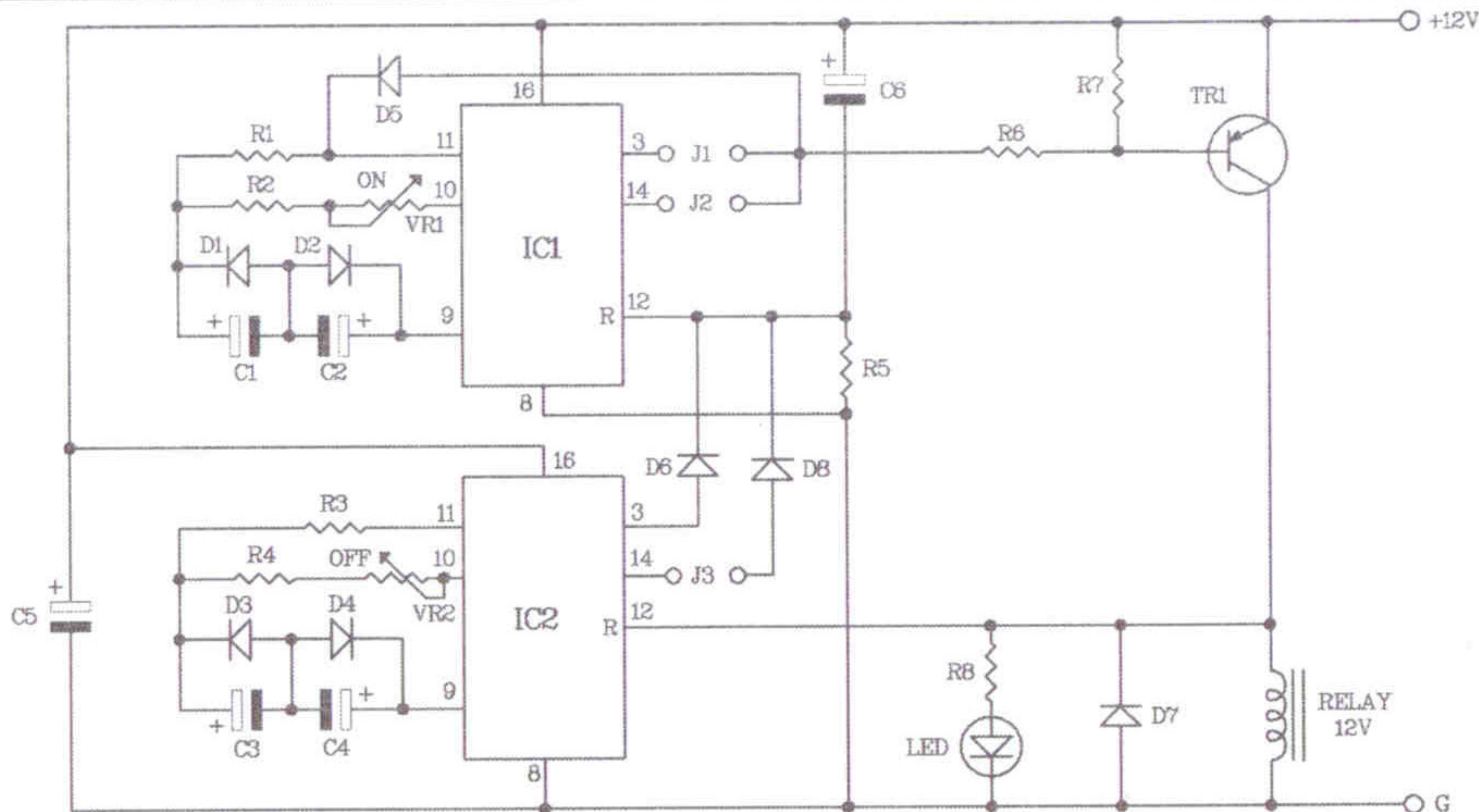
Figure 2. The circulated on-off switch circuit
